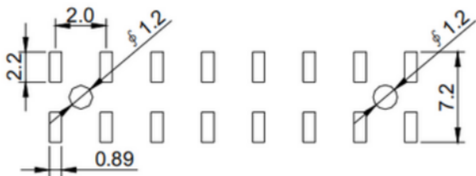
PCB LAYOUT
